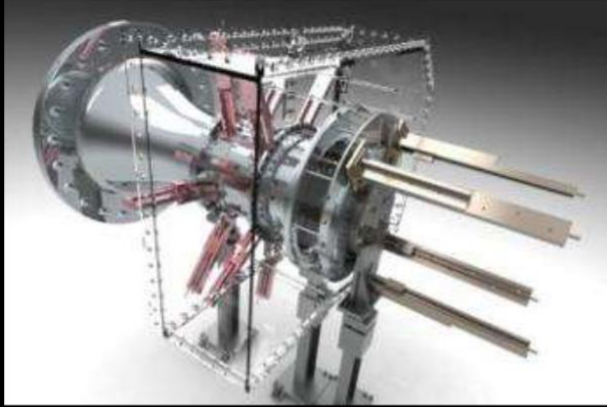
Diffuser
