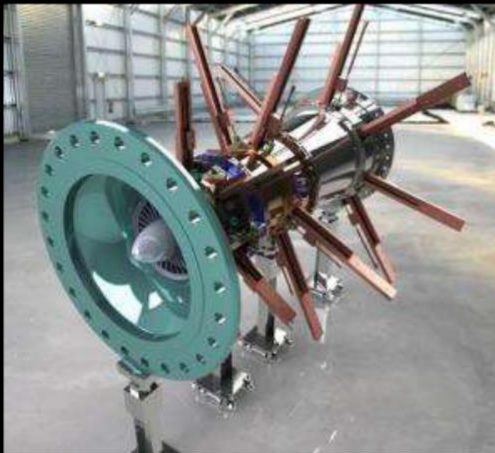
Advanced Diffuser
